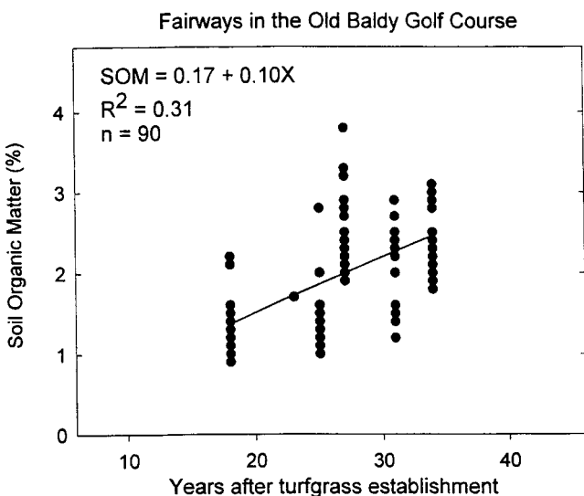
Fig. 3. Soil organic matter changes (to 15.2 cm) in fairways of the Old Baldy Golf Course, Wyoming.
