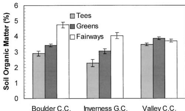
Fig. 4. The soil organic matter in greens, fairways, and tees of Boulder Country Club, Inverness Golf Course, and Valley Country Club. Turf in the tested sites was >25 yr old. Vertical lines represent standard errors.
