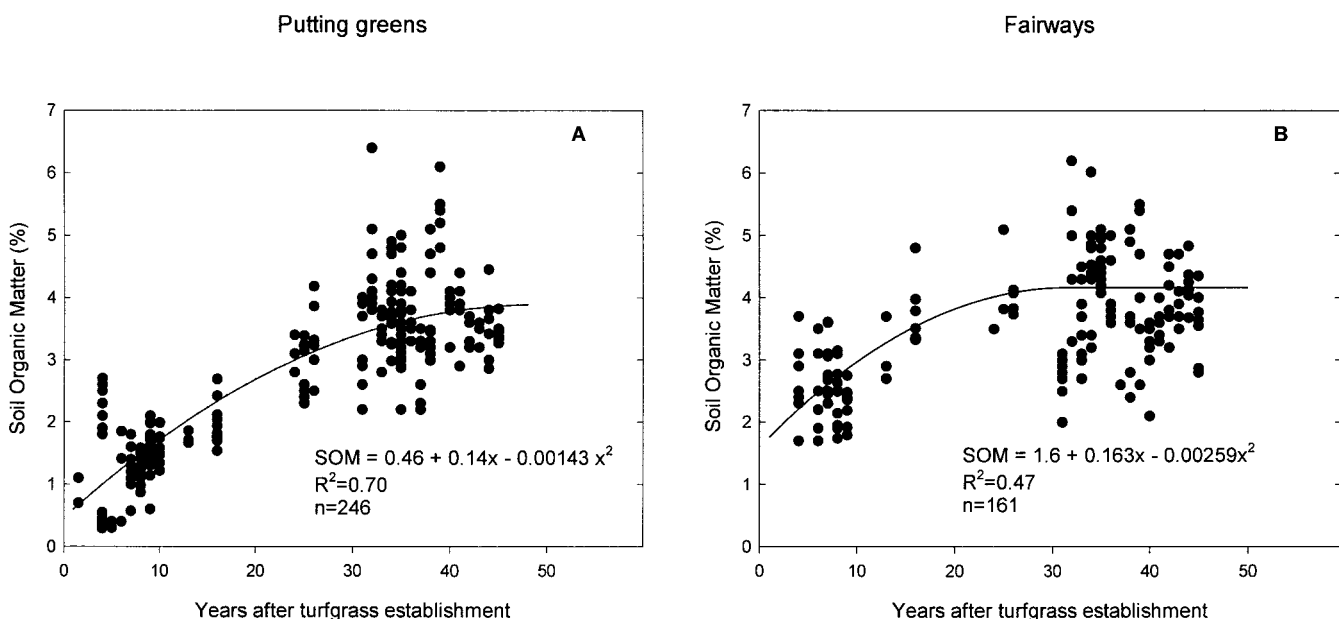
Fig. 1. Changes in soil organic matter with time since turfgrass establishment in (A) putting greens of 16 golf courses in Colorado and (B) fairways of 13 golf courses in Colorado. Data were based on soil-testing results from these golf courses sampled to 11.4-cm depth.
